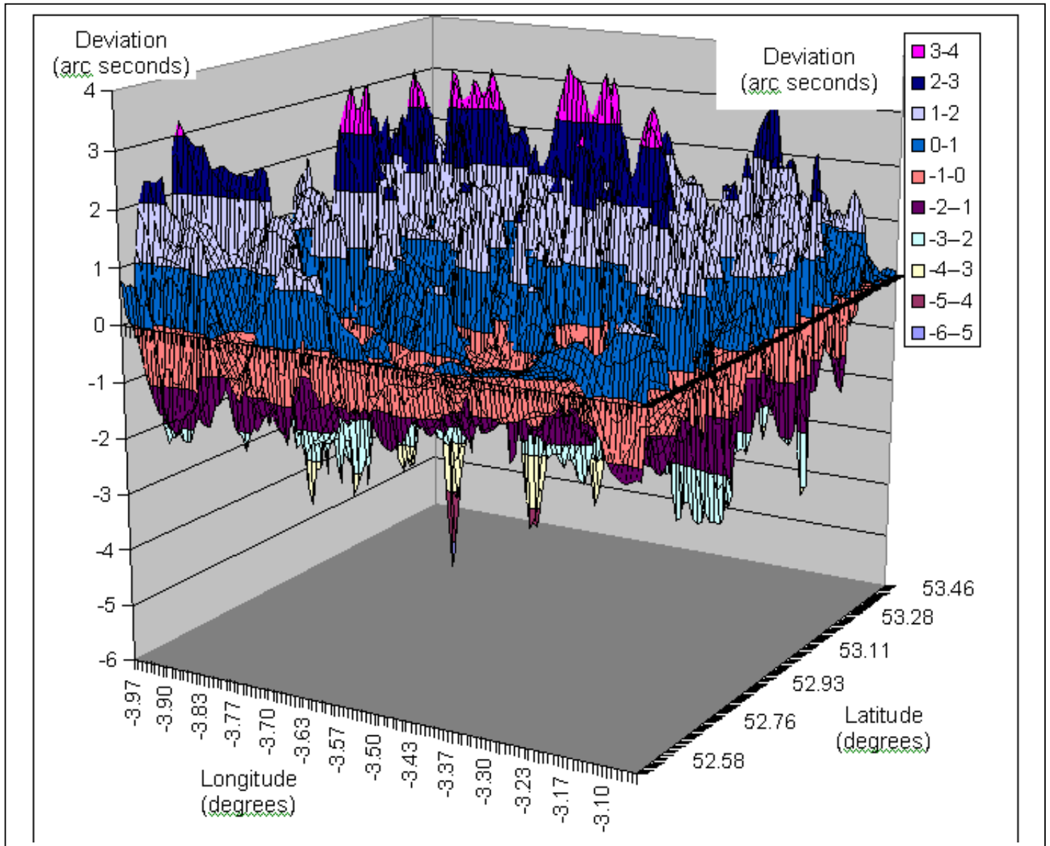
Aviemore Block north-south topographic-isostatic deviation
